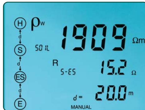
The Wenner test displays test lead connection, soil resistivity test results ( \rho ), electrode spacing and resistance.
