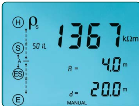
The Schlumberger test displays test lead connection, soil resistivity test results ( \rho ) and electrode spacing.
